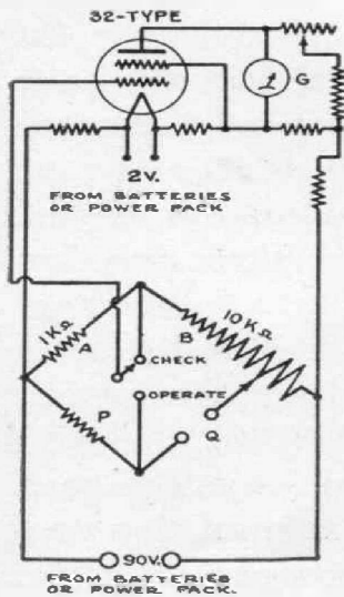
FIGURE 2. Schematic diagram for the TYPE 544-A Megohm Meter
