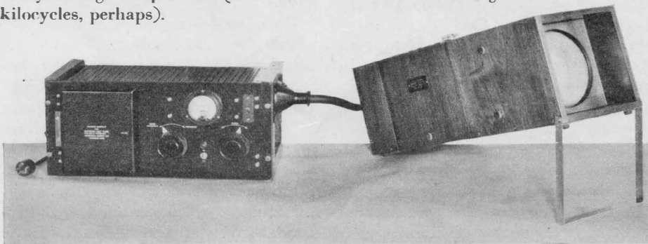
FIGURE 2. The power-supply unit, tube, and TYPE 579-A Tube Mounting
