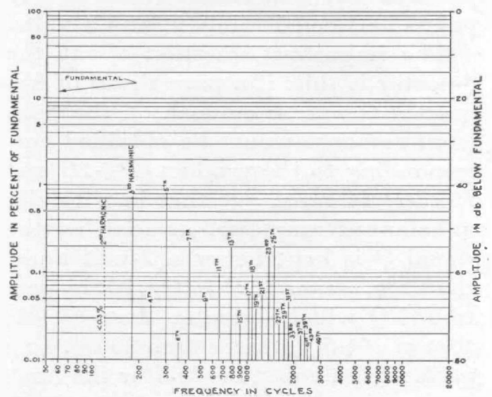
FIGURE 4. Wave analysis on a commercial 60-cycle circuit for components up to the 50th harmonic. The relative amplitudes were obtained directly from the analyzer's voltmeter by adjusting the fundamental for a deflection of 100 volts
