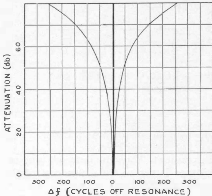
FIGURE 5. Over-all characteristic of the 50,000-cycle quartz-crystal filter in the wave analyzer. This filter passes the upper side-band only
