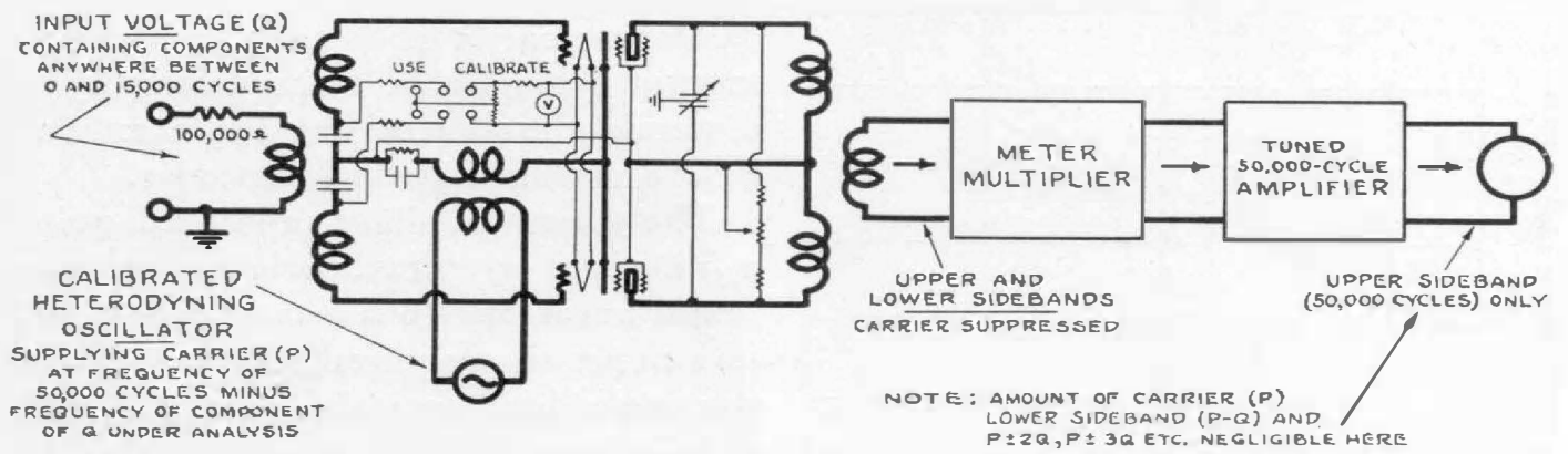
FIGURE 2. The TYPE 636-A Wave Analyzer has better frequency discrimination as well as other advantages over the conventional tuned-circuit analyzer
