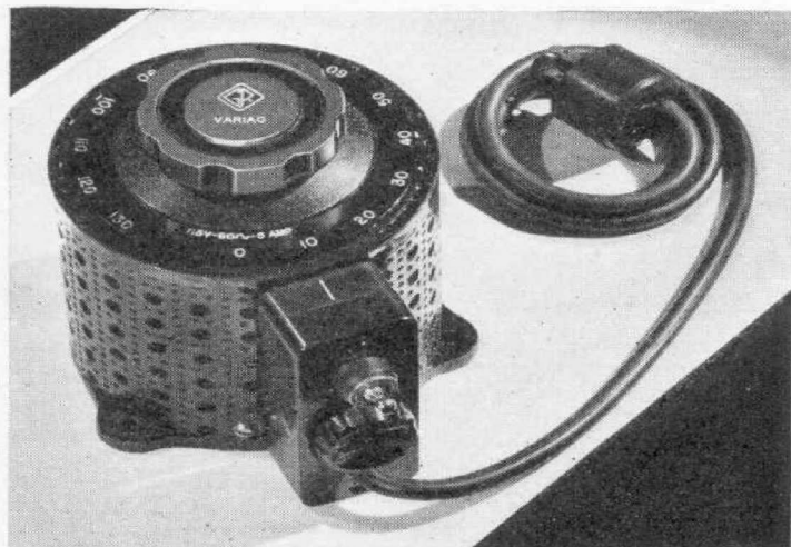
The TYPE 200-CM Variac is an adjustable auto-transformer delivering voltages between 0 and 130 volts from the 115-volt line. (Patent applied for)
