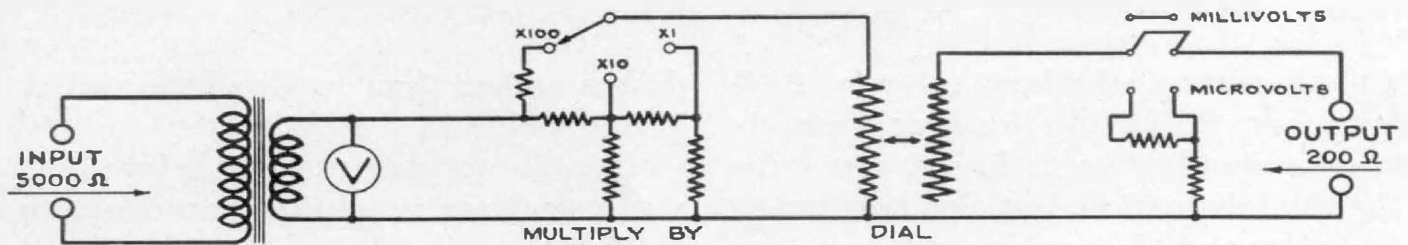
Schematic diagram of the TYPE 546-A Audio-Frequency Microvoltmeter. The open-circuit voltages shown by the calibration are obtained when the voltmeter reads 2 volts
